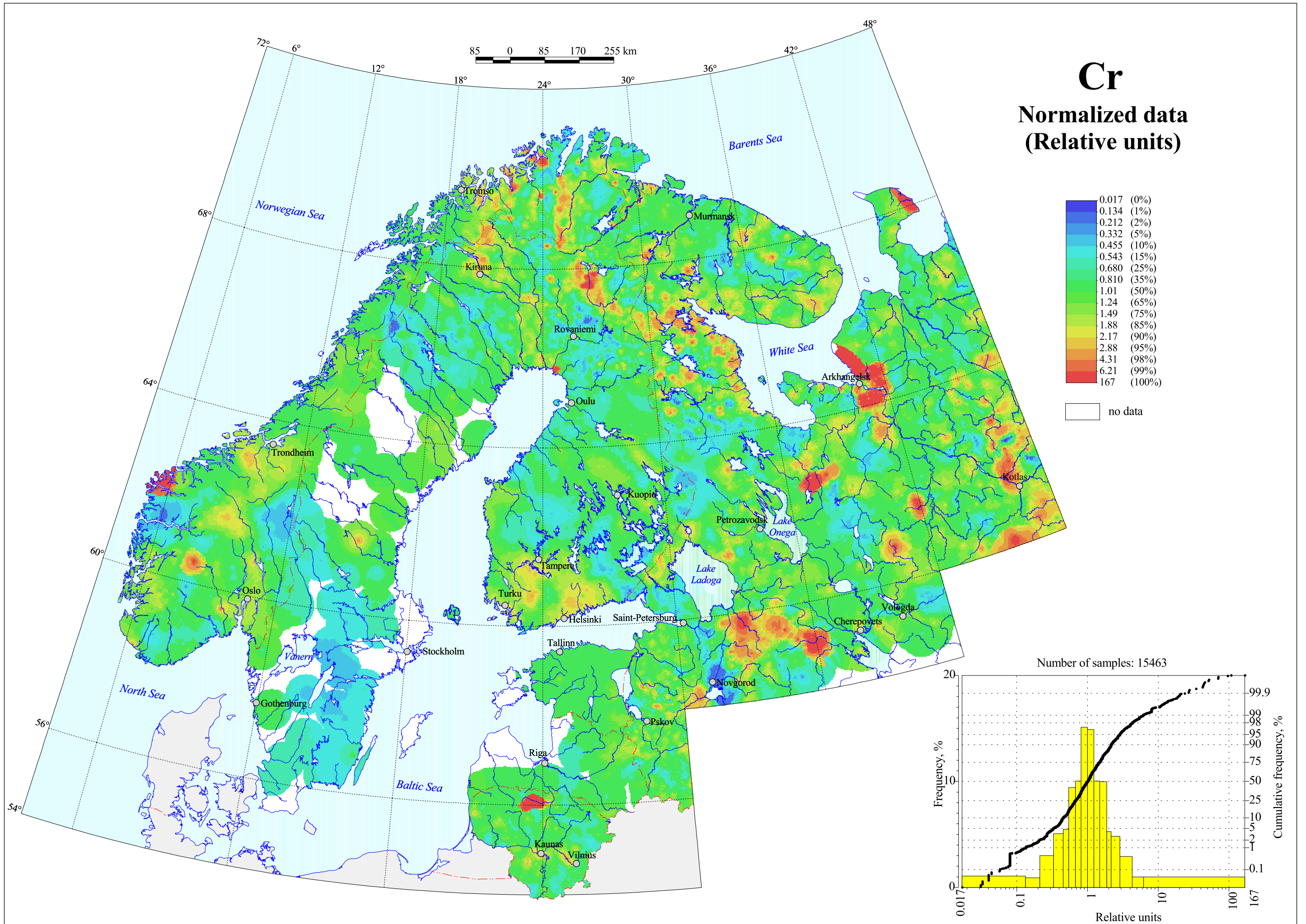
Chromium in Stream Sediment
